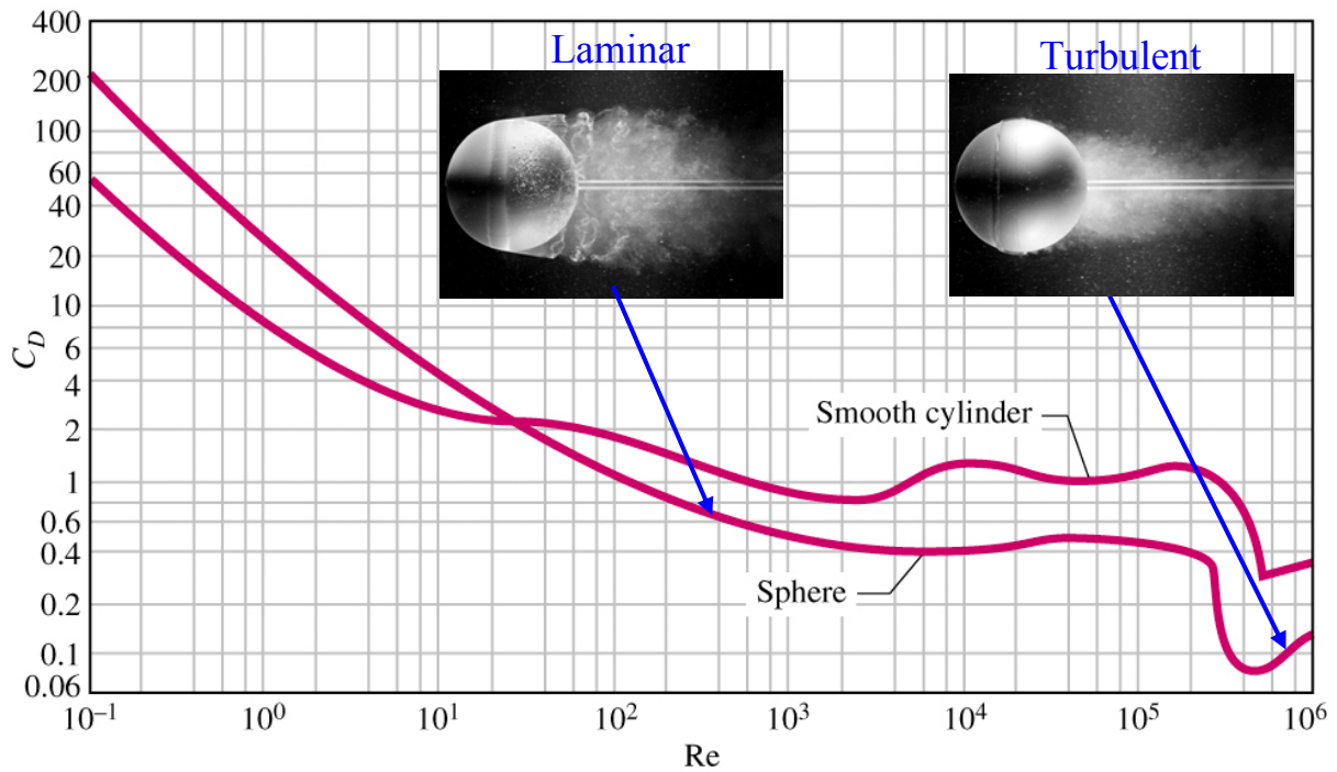
Figure 11-34. Average drag coefficient for cross-flow over a smooth circular cylinder and a smooth sphere.
